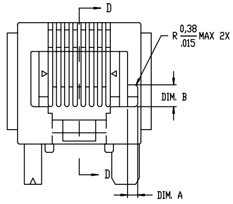
KEYED STYLE
